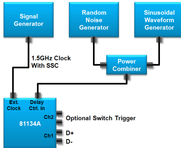
Figure A-2: Use of Keysight 81133/4A as the SSG
