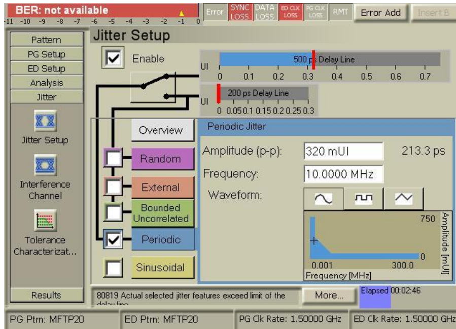
Figure E-4: J-BERT N4903A Jitter Setup Screen (DJ)
