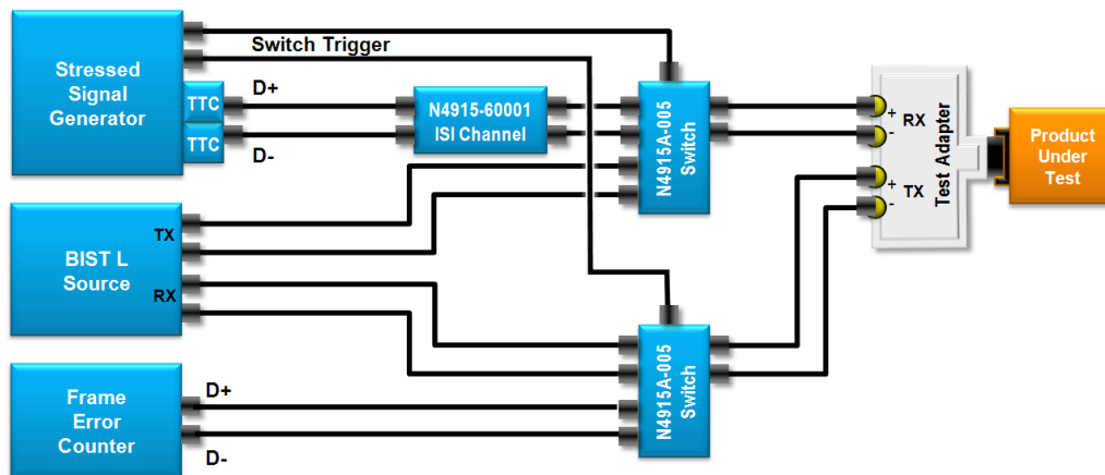
Figure A-1a: Basic RSG-01/02/03/05/06 Test Setup with separate BIST L Source
