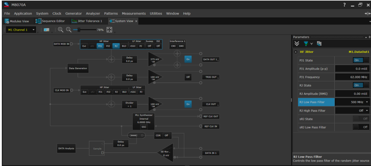
Figure F-3: J-BERT M8020A HF Jitter Setup Screen
