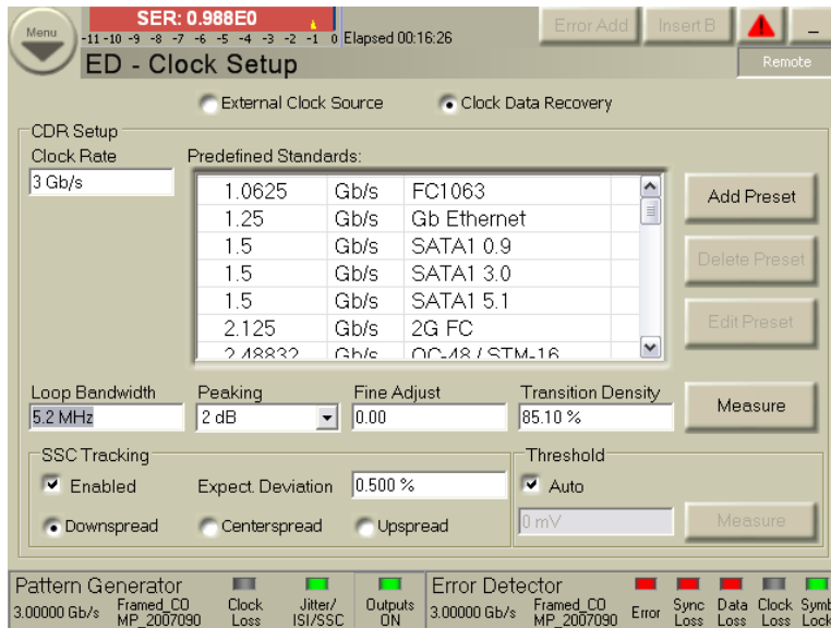
Figure M-3: J-BERT Error Detector Clock Setup Menu
