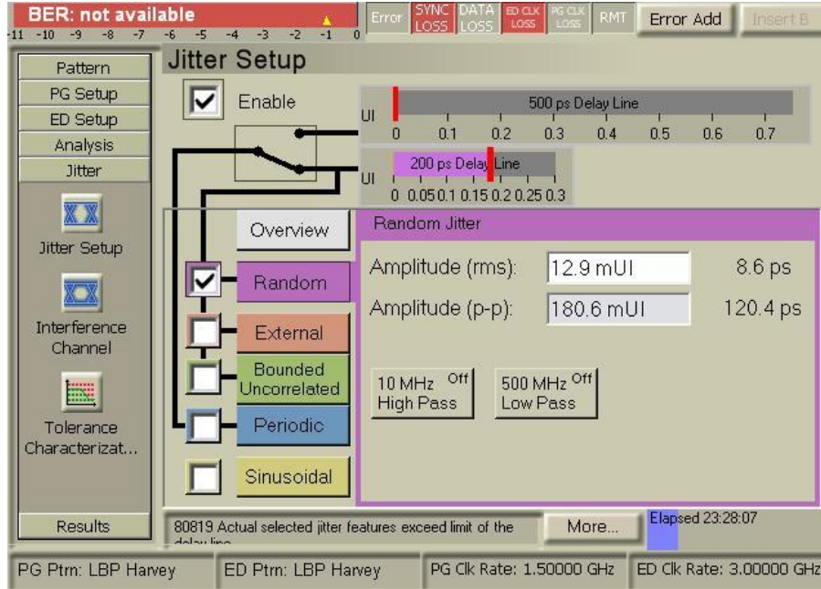
Figure E-3: J-BERT N4903A Jitter Setup Screen (RJ)
