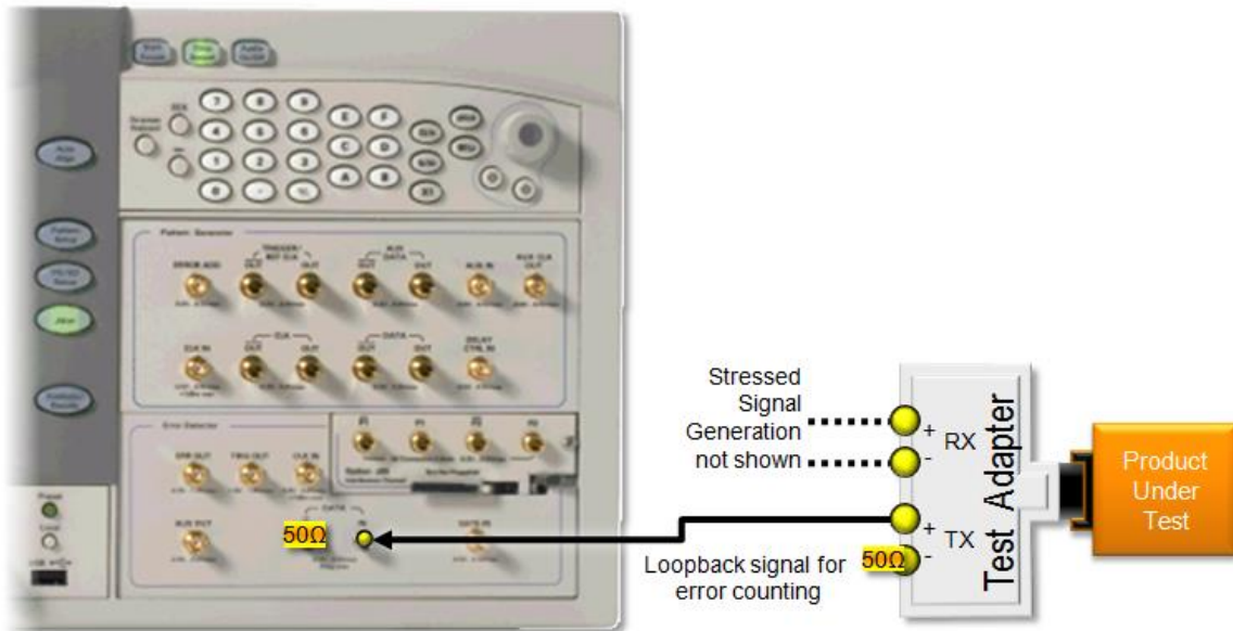
Figure M-1: Connection Diagram Using J-BERT Error Detector as the Frame Error Detector
