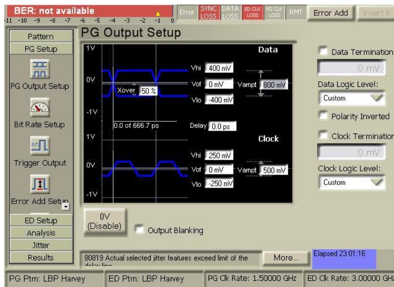
Figure E-2: J-BERT N4903A Amplitude Setup Screen
