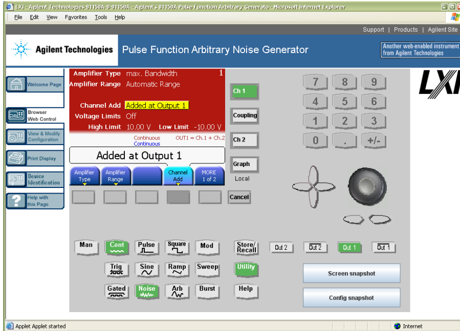
Figure L-3: Keysight 81150A remote interface with channel add feature turned on.
