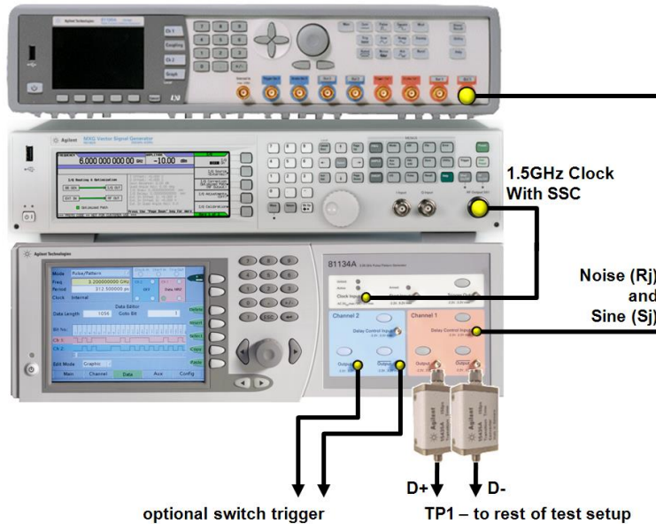
Figure L-1: Keysight 81134A Pulse and Pattern Generator, Keysight 81150A Pulse Function Arbitrary Noise Generator, and Keysight N5182A MXG RF Vector Signal Generator
