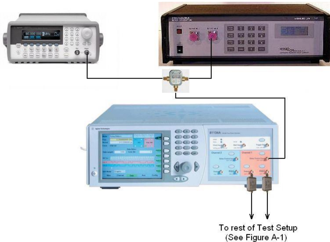
Figure G-1: Keysight 81134A Pulse and Pattern Generator, Keysight 33250A Function/Arbitrary Waveform Generator, and Noisecom PNG-7110 Noise Generator
