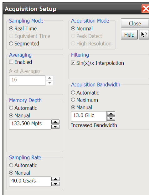
Figure B-2: Acquisition Settings for Gen1
