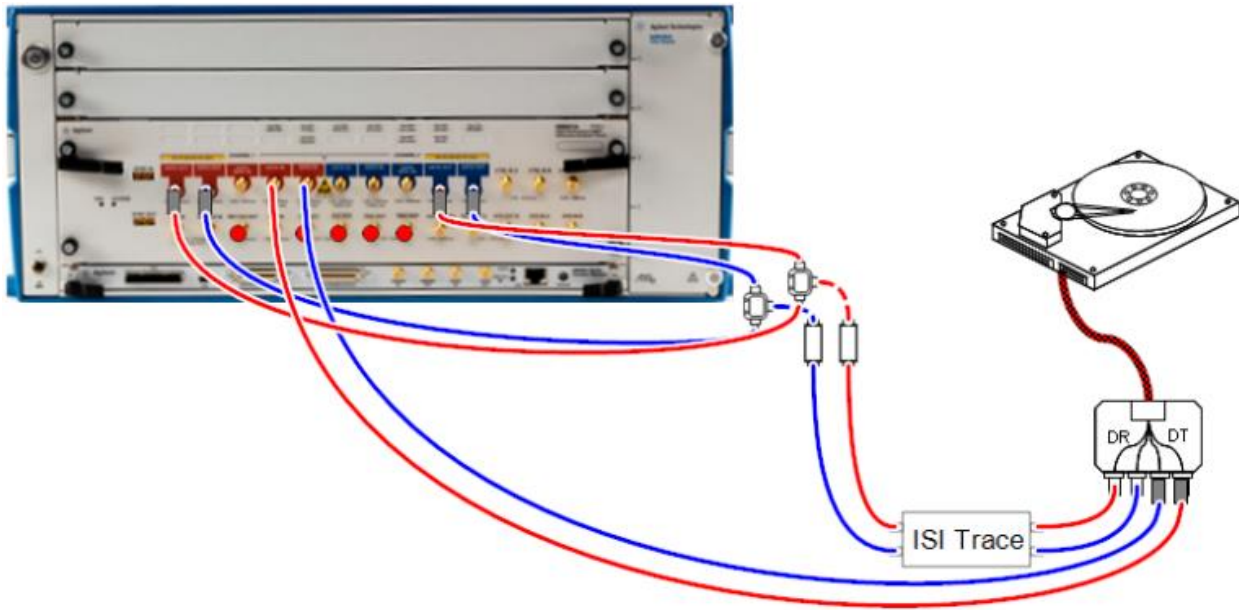
Figure F-1: J-BERT M8020A based SATA RSG test setup
