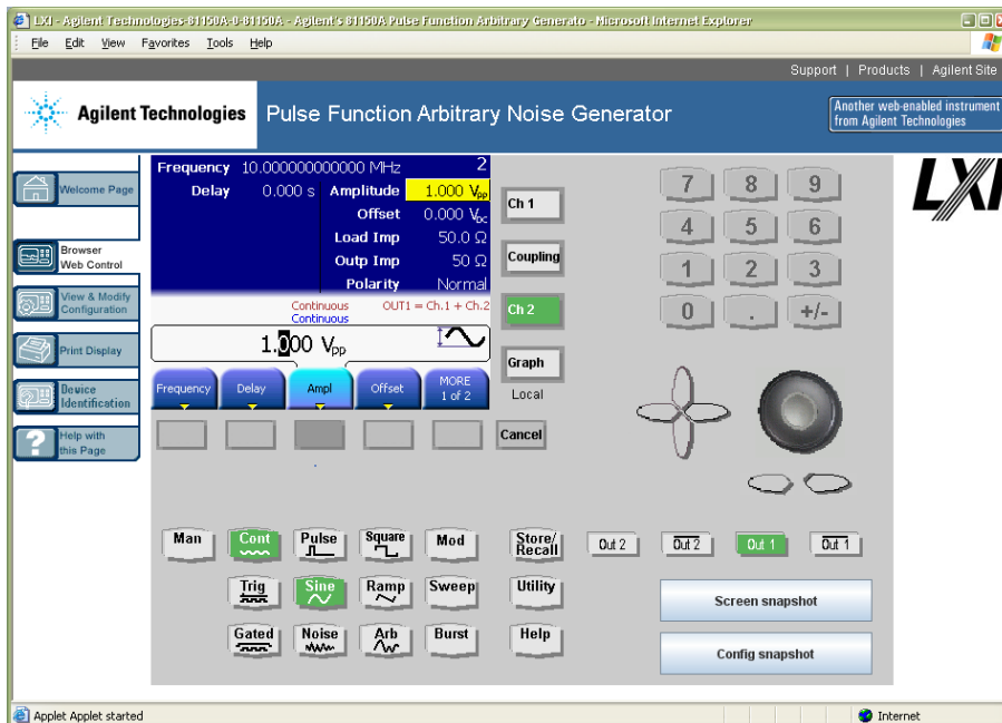
Figure L-4: Keysight 81150A remote interface with sinusoidal waveform configuration for channel 2 shown.
