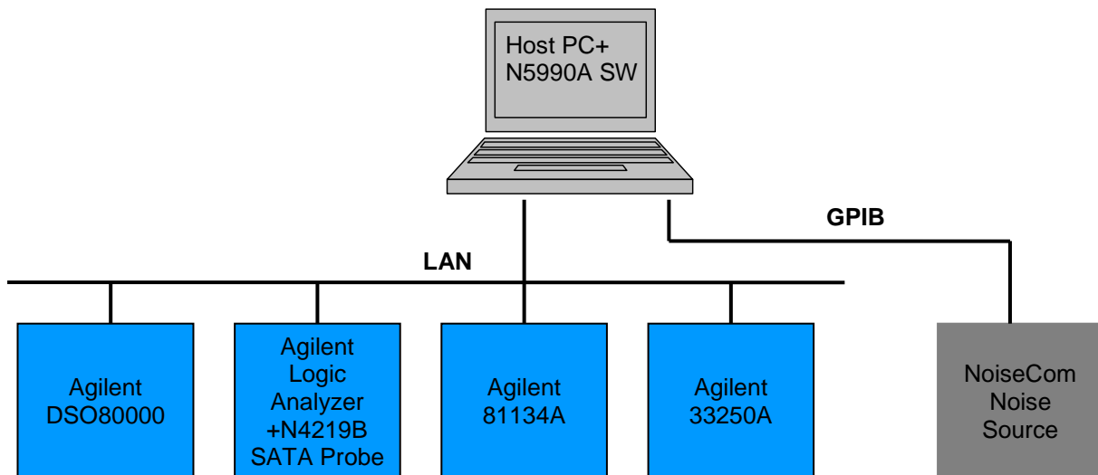
Figure K-1: Test Equipment Network Diagram
