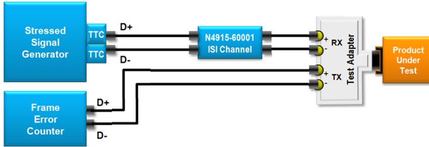
Figure A-1b: Basic RSG-01/02/03/05/06 Test Setup. SSG performs BIST L training
