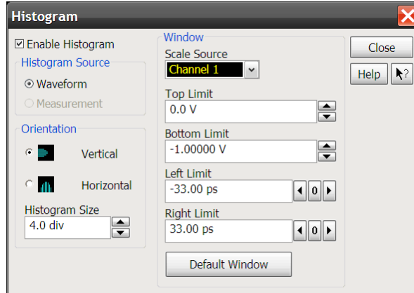
Figure B-5: Gen1 Histogram Settings for Lower Inner Eye
