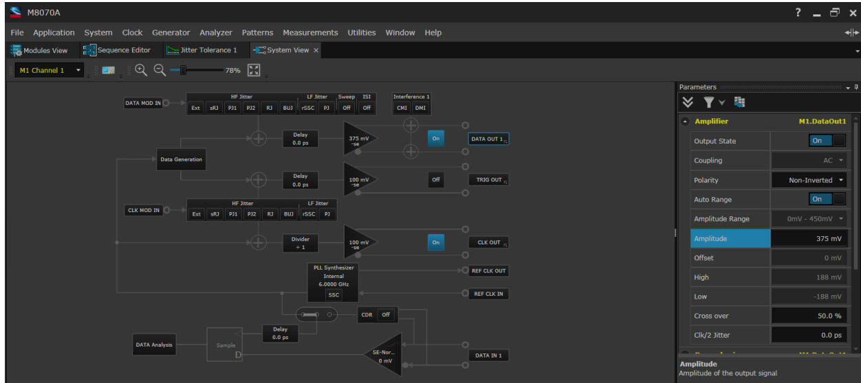
Figure F-2: J-BERT M8020A Data Out1 Amplifier Setup Screen
